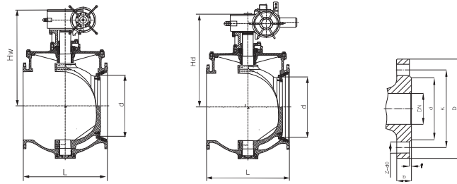
PN1.0MPa主要外形和连接尺寸 Main connection and external dimensions
